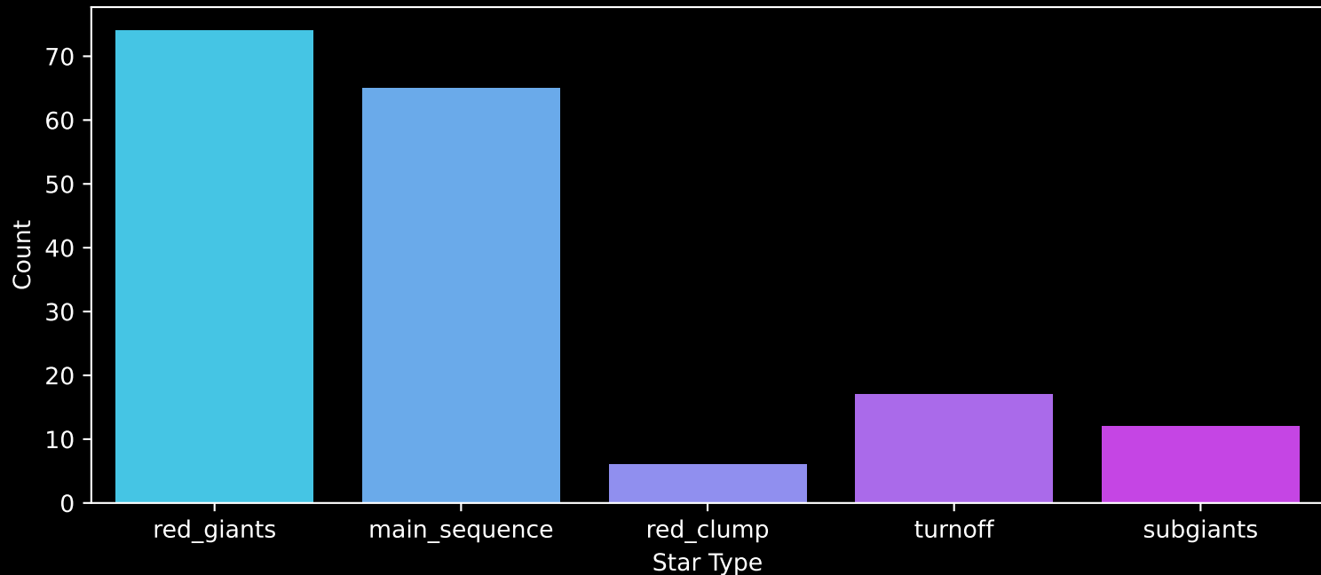
APOGEE DR17 Field: [150-45] Count plot of Star Type
