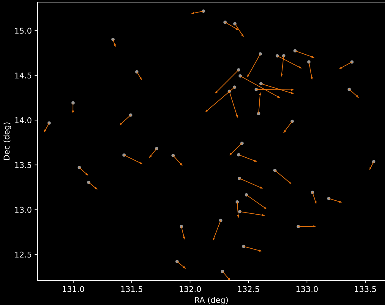
APOGEE DR17 Cluster 2 Proper Motion Vectors (n=44)
