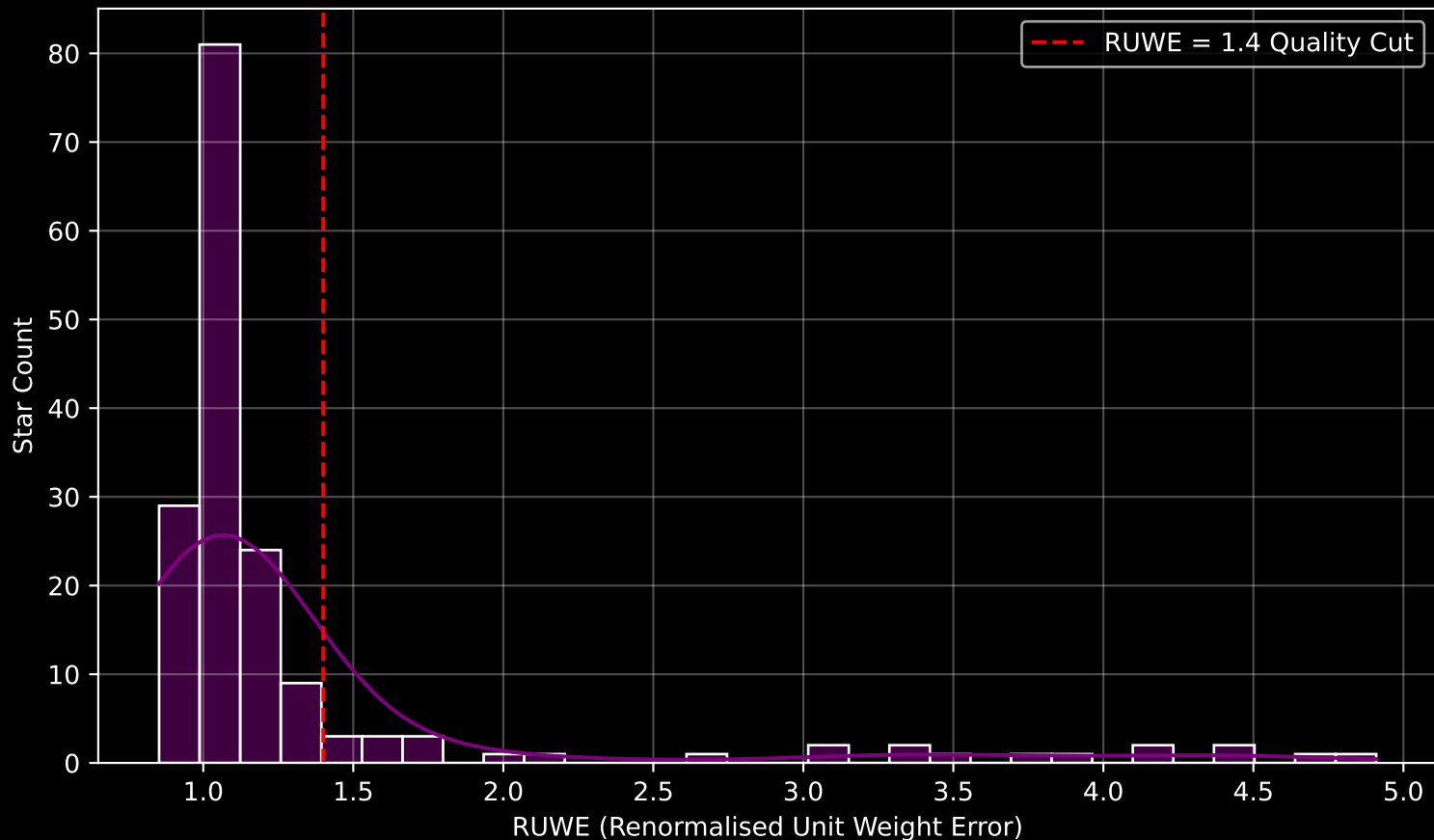
GAPOGEE DR17 Field [150-45] RUWE Distribution (n= 168)
