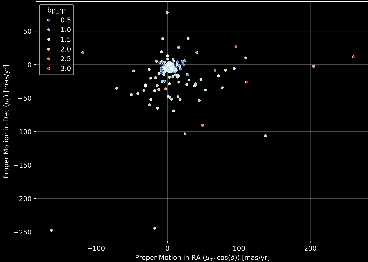
APOGEE DR17 Field: [150-45] Proper Motion Diagram (n= 174)
