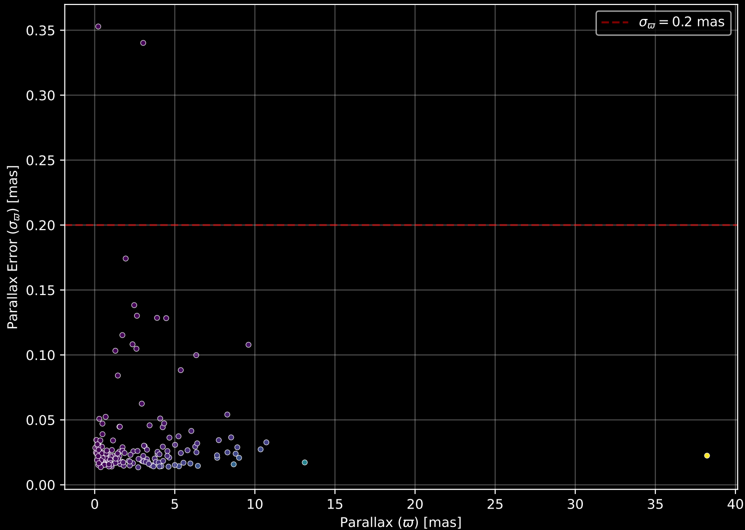
APOGEE DR17 Field: [150-45] Parallax Quality (n= 174)
