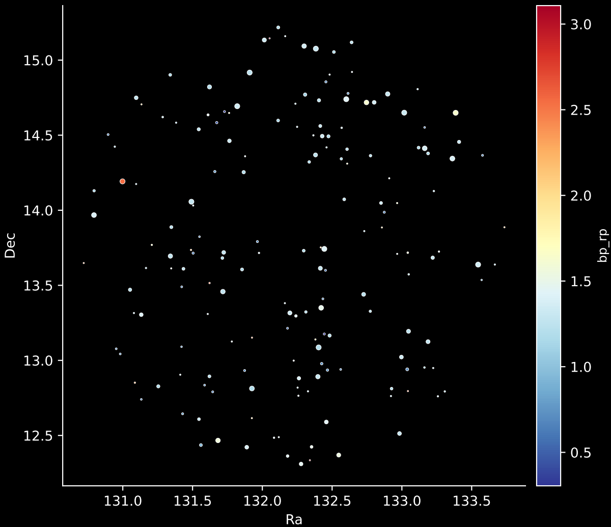
APOGEE DR17 Field: [150-45] Stars: 174
