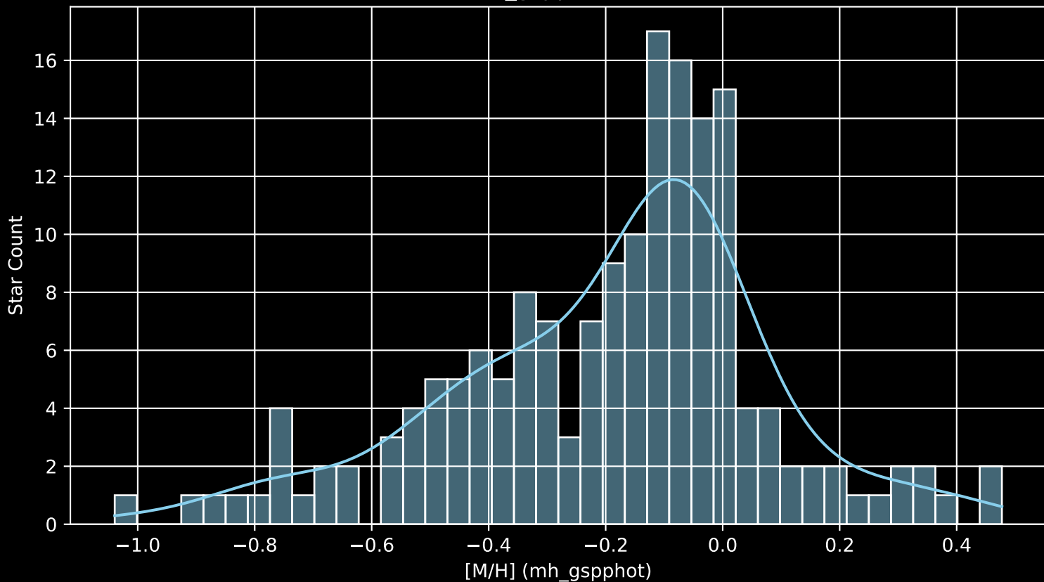
APOGEE DR17 Field: [150-45 [M/H] (mh_gspphot) (n= 171)
